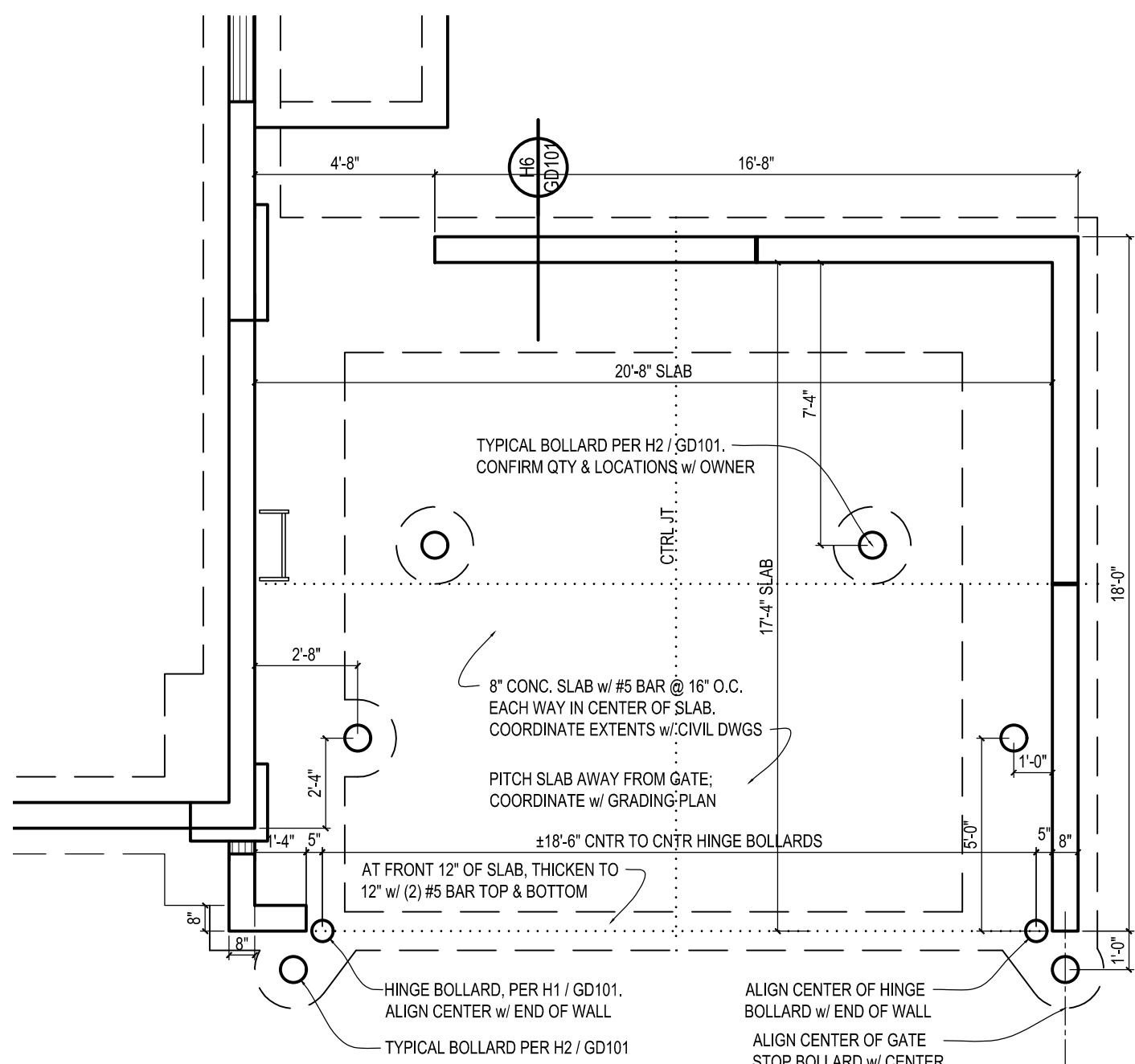
C2 FOUNDATION PLAN SCALE : 1/4" = 1'-0"
