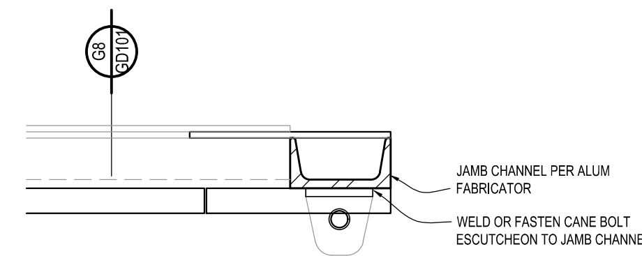
E8 SECT @ GATE MTG STILES SCALE : 3" = 1'-0"
