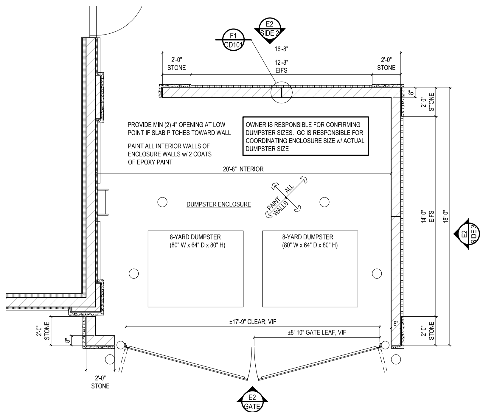
C3 FLOOR PLAN SCALE : 1/4" = 1'-0"
