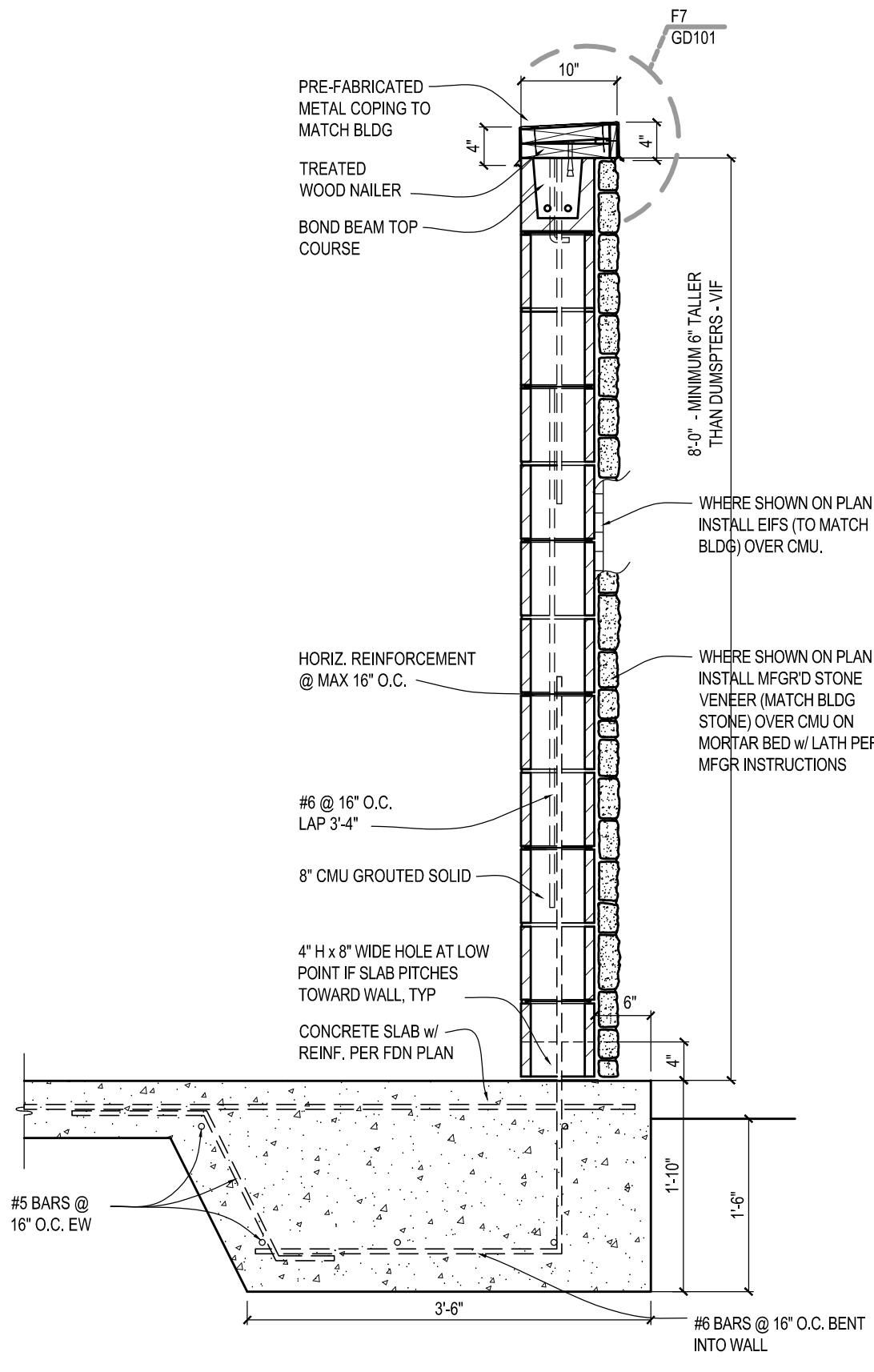
H6 ENCLOSURE WALL SCALE : 3/4" = 1'-0"
