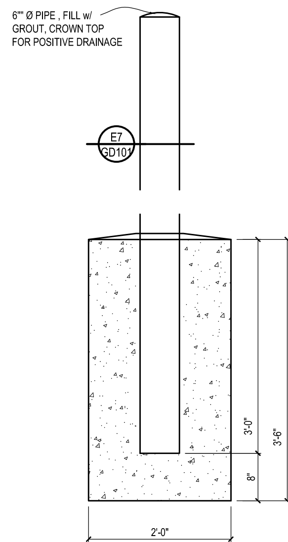
H1 HINGE BOLLARD SCALE : 3/4" = 1'-0"
