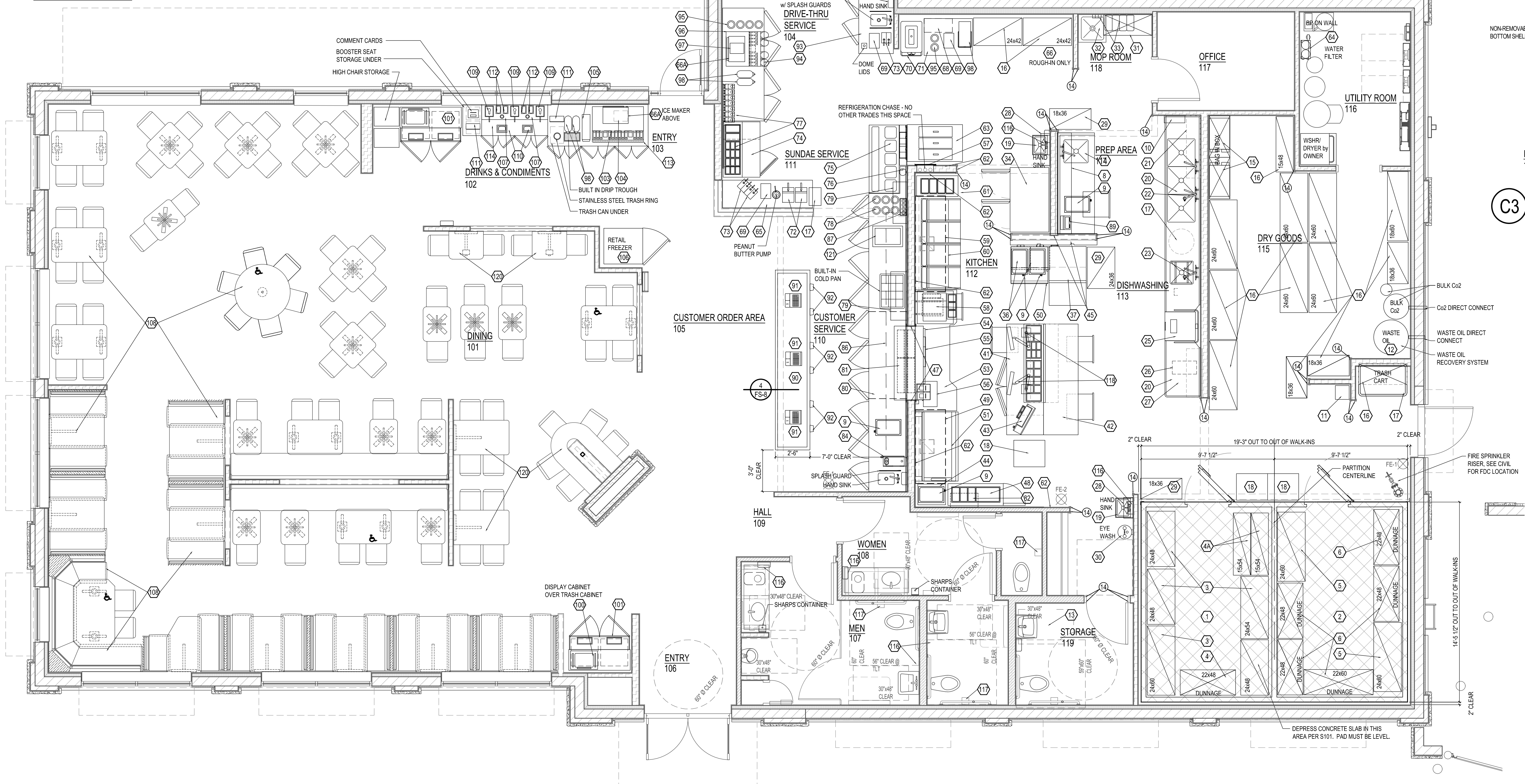
FOODSERVICE PLAN SCALE: 1/4" = 1'-0"
