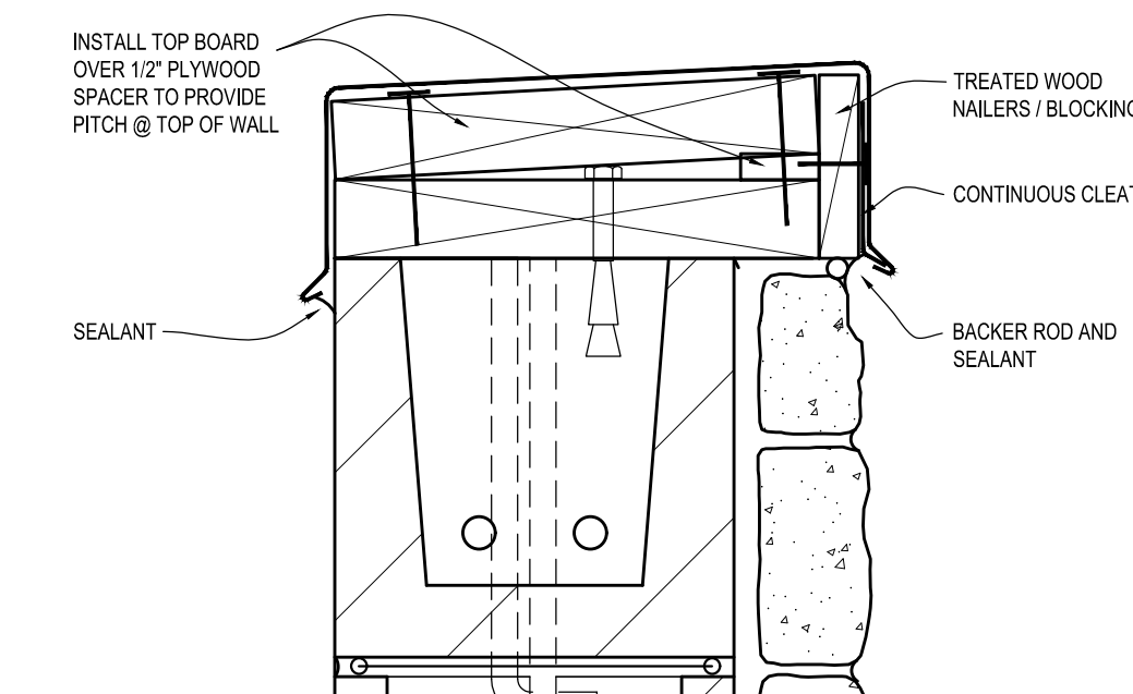
F7 DETAIL SCALE : 3" = 1'-0"
