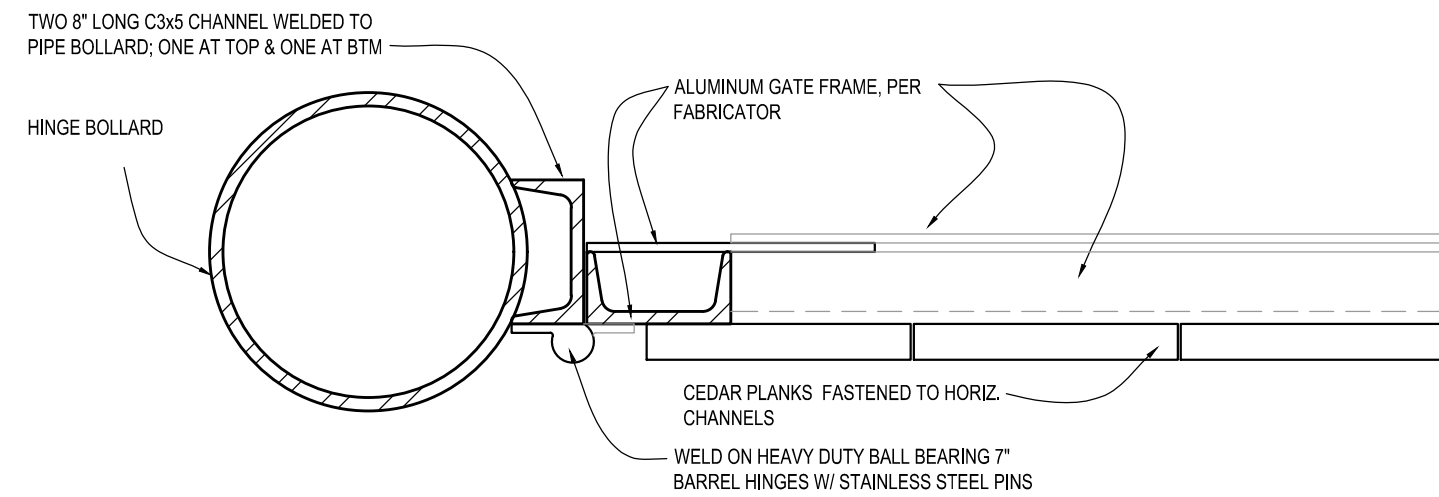
E7 HINGE DETAIL SCALE : 3" = 1'-0"
