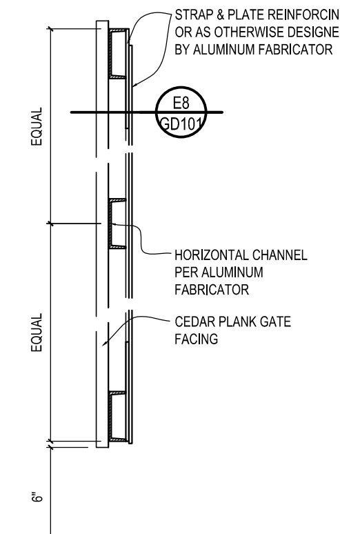
G8 DETAIL SCALE : 1 1/2" = 1'-0"
