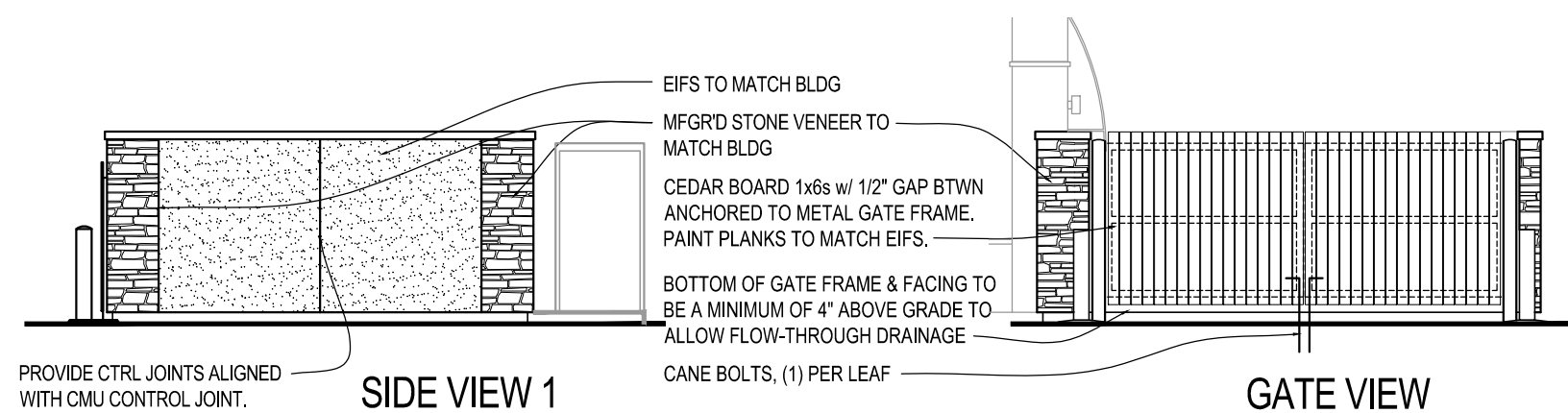
E2 ENCLOSURE ELEVATIONS SCALE : 1/8" = 1'-0"
