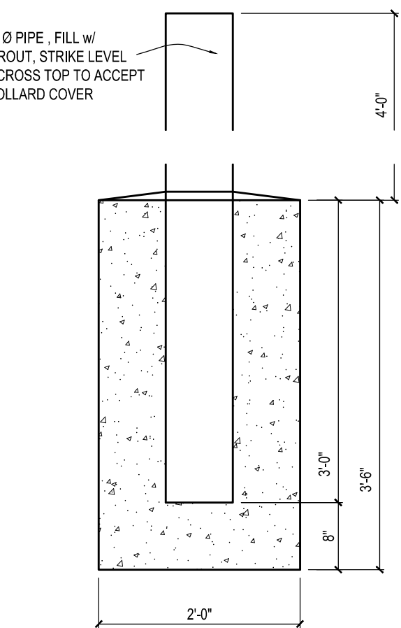
H2 BOLLARD SCALE : 3/4" = 1'-0"
